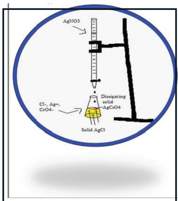
Fig1: Conventional Chloride ion estimation titration setup
